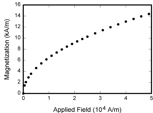
Figure 1: Magnetization as a function of applied field.
